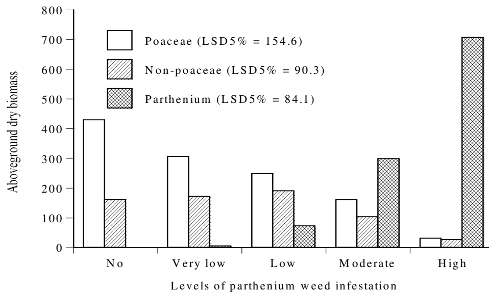
Figure 1. Above-ground dry biomass ( \text{g m}^{-2} ) of Poaceae, non-Poaceae species and parthenium weed at five P. hysterophorus infestation levels
