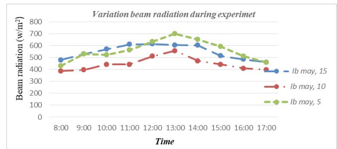
Figure 4. Variation of solar radiation results from measured temperatures by the black painted horizontal plate.
