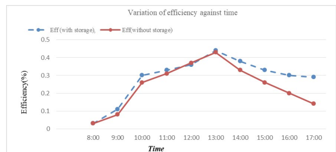
Figure 9. Variation of collector efficiency with time.
