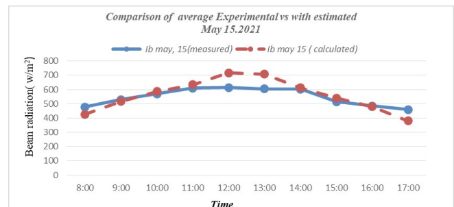
Figure 5. The comparison of experimental data with calculated.
