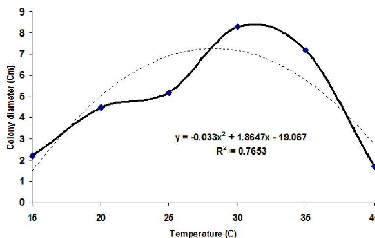
Figure 4. Experimental (solid line) and model (dash line) growth rate values of 56 isolates of Macrophomina phaseolina at different temperature in 5 days. Values are the mean of three replications.
