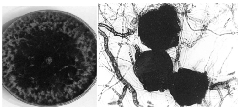
Figure 3. Colony of Macrophomina phaseolina recovered from olive plants collected from olive nursery in Gorgan region, Golestan province (left) and the microsclerotia under compound microscope (right, 40X).
