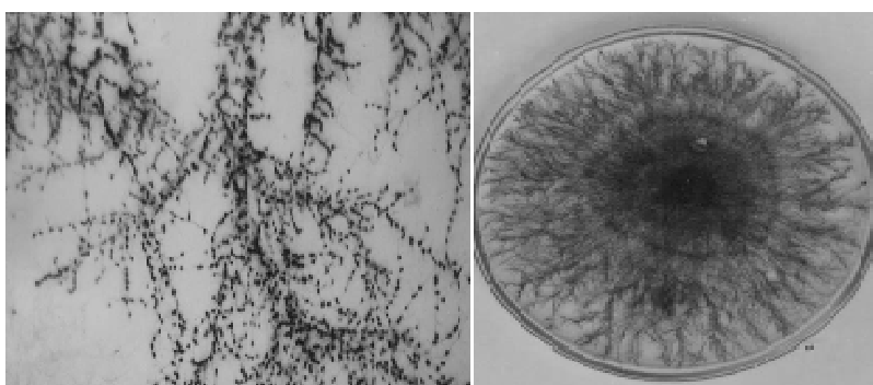
Figure 5. Growth patterns of Macrophomina phaseolina of colony (right) and microscerotia (left) on a minimal medium containing 120 mM potassium chlorate.
