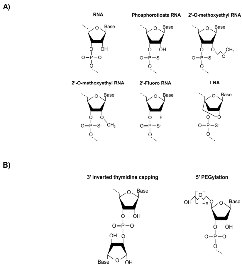
Figure 2. Chemical modifications. Diagram shows the most common chemical substitutions incorporated into synthetic oligonucleotides aimed to improve their pharmacodynamic properties. Pre-SELEX ( A ) and post-SELEX ( B ) modifications mentioned throughout the text are included. PEG, polyethylenglycol.
