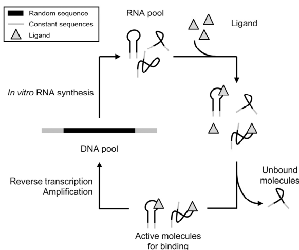
Figure 1. In vitro selection methods. A) General scheme of an in vitro selection procedure involving an RNA library. An RNA population containing active and inactive variants is subjected to a selective pressure. Active RNA molecules are selectively recovered and reverse transcribed. Amplification of the Cdna templates generates a DNA pool, which is transcribed to yield a new RNA population that can be sampled and subjected to further selection rounds if required. B) SELEX process. Identification of RNA aptamers targeting a specific ligand by the application of an in vitro selection method. Figure adapted from (Romero-López et al., 2007). Suppression of transcription and reverse transcription steps allows for the isolation of active DNA oligonucleotides.
