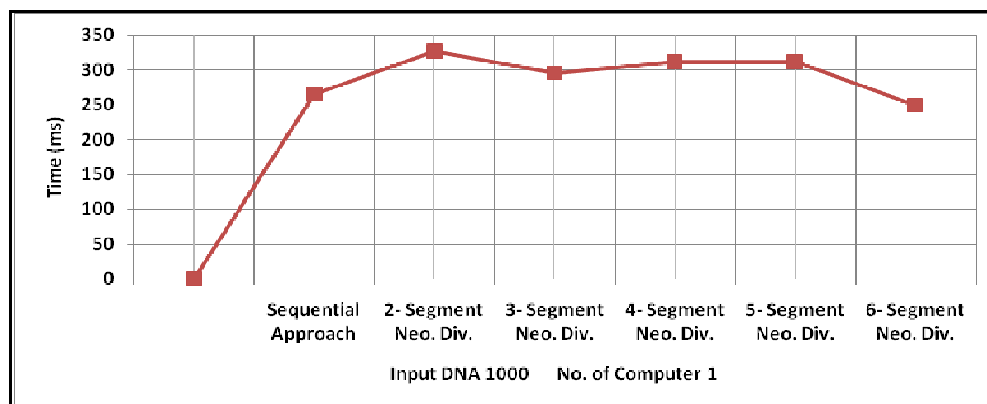
Figure 7. Effect of Data size on using Single Computer
