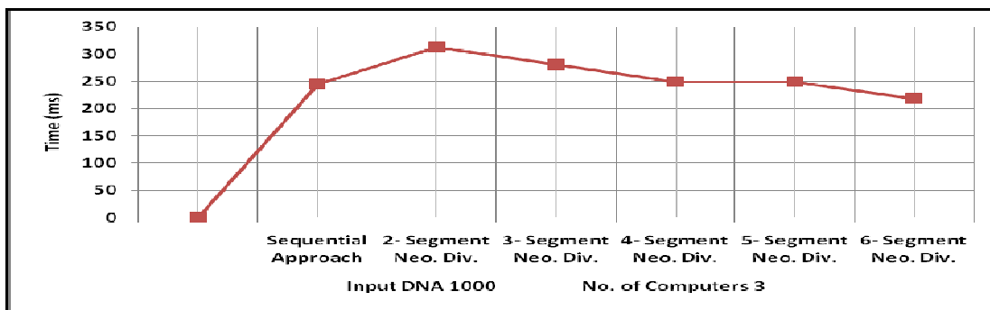
Figure 9. Effect of Data size on using Three Computers
