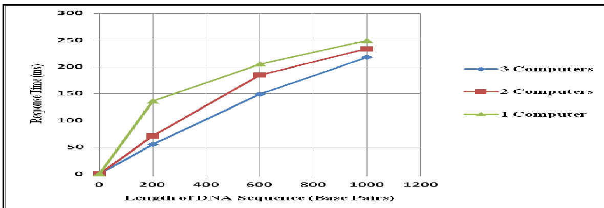
Figure 10. Effect of Data Size on Computation Time
