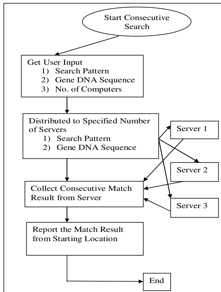
Figure 3. Flow Diagram for Client Side Implementation
