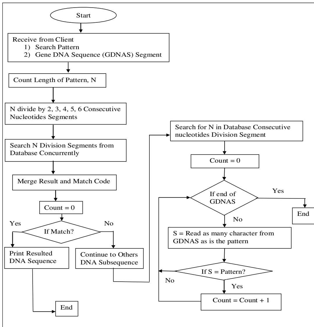
Figure 4. Flow Diagram for Consecutive Search Pattern from Server
