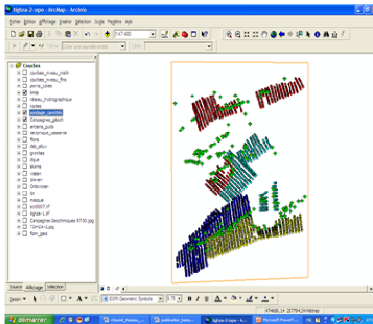
Figure 3. Geochemical profiles and Cores drilling maps
