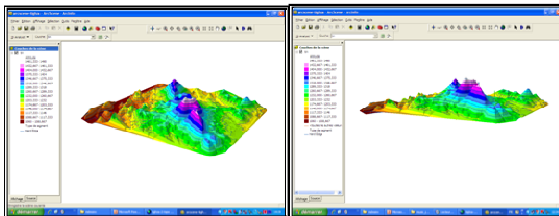
Figure 4. Digital Elevation Model (DEM) of the Tighza mining district
