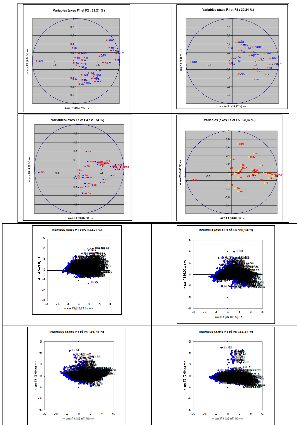
Figure 8. Projection of the variables and individuals according to the first four factorial designs absorbing the maximum total variance
