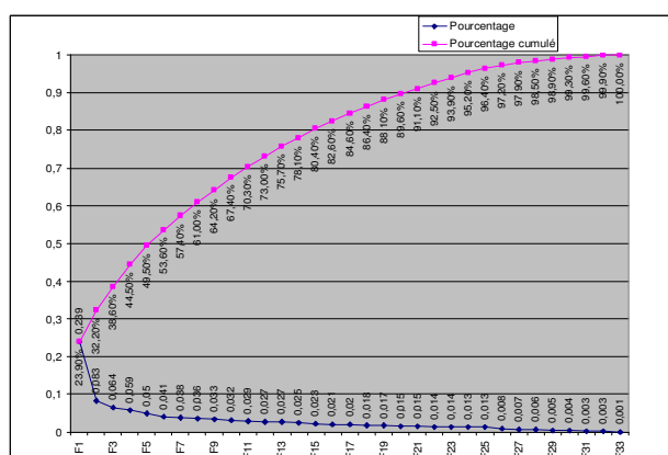
Figure 7. Graphic of the percentages and cumulative percentages of the absorbed variance by its eigenvalues
