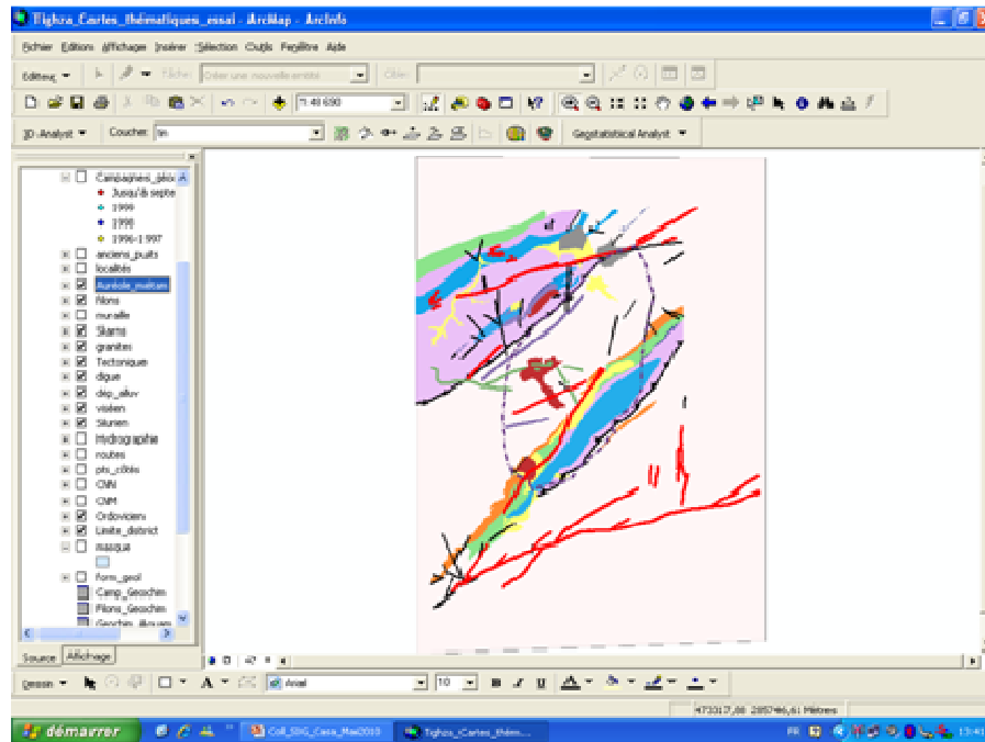
Figure 2. Geological and metallogenic maps developed by using the GIS tool
