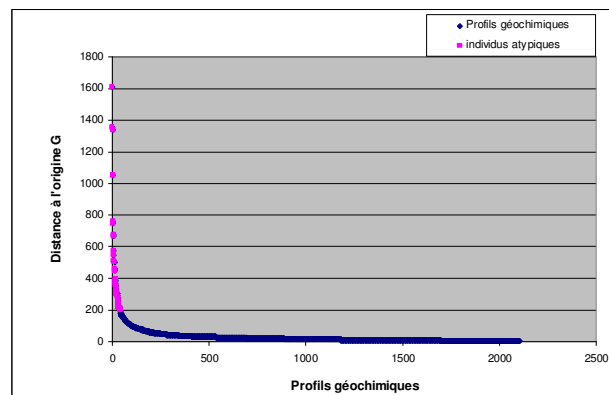
Figure 6. Distance from the origin G of the geochemical profiles
