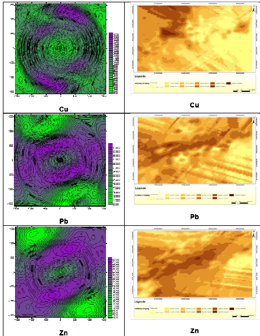
Figure 10. Variographic maps (on the left) and Ordinary kriging maps of some chemical (on the right)
