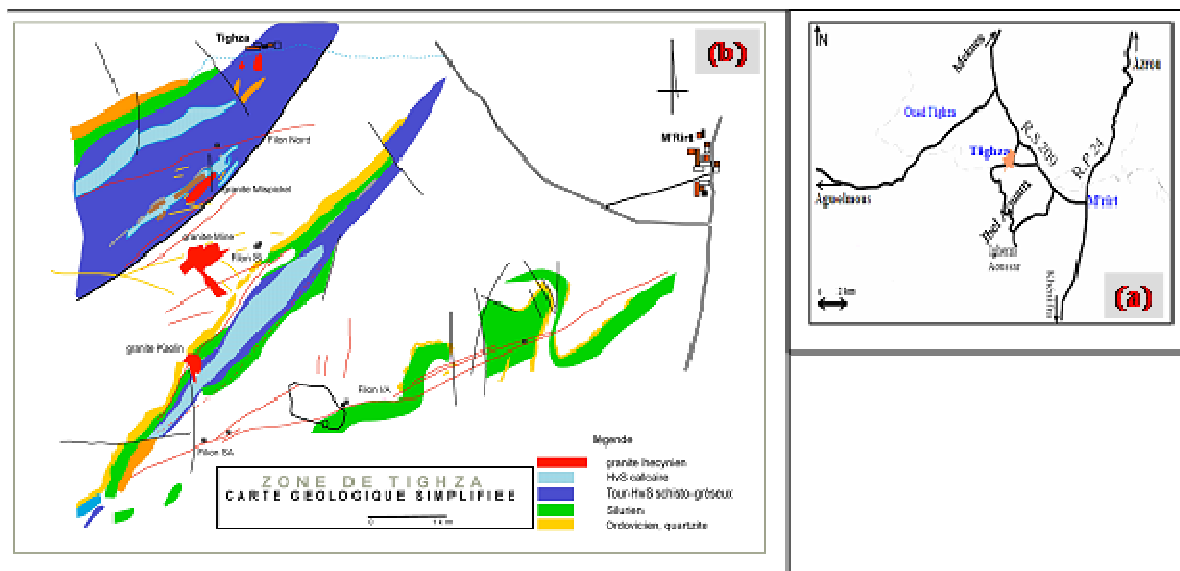
Figure 1. Geographic location (a) and geological context of Tighza mining district (b)
